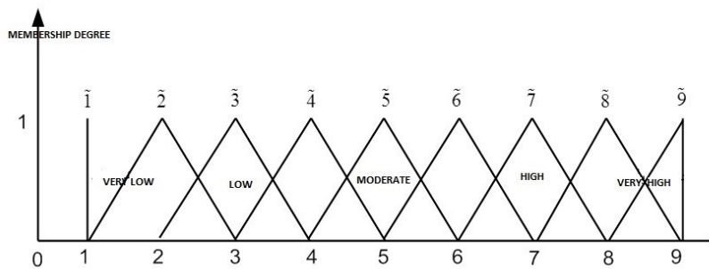
Fig. 2. Used fuzzy numbers in this research
